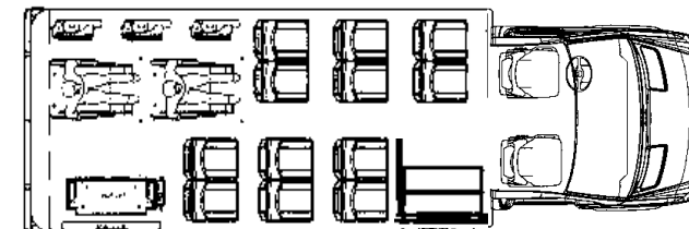
⑤ Side ADA Two wheelchairs Seating 14+6, 2w/c
